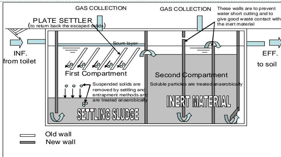
Figure (3) modified septic tank USBR
