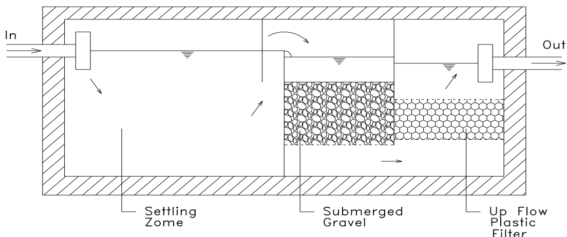
Figure (4) Applied modified septic tank
